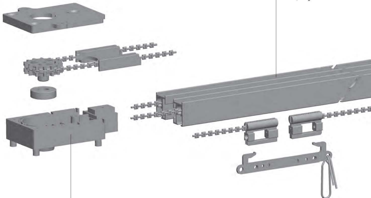
3135 3- Schiene gerade / Rail droit / Track, straight
